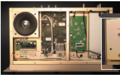
RX-340 Top view
