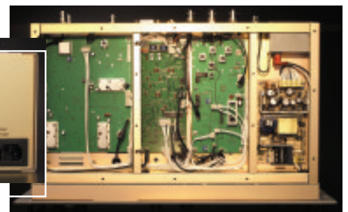
RX-340 Bottom view
